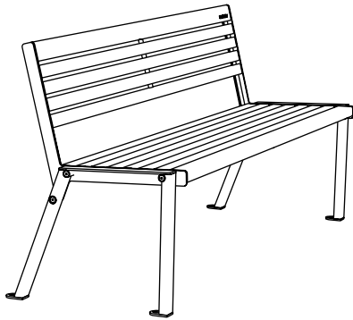
Klaar Wood bench with backrest, without armrests - KLWB190
